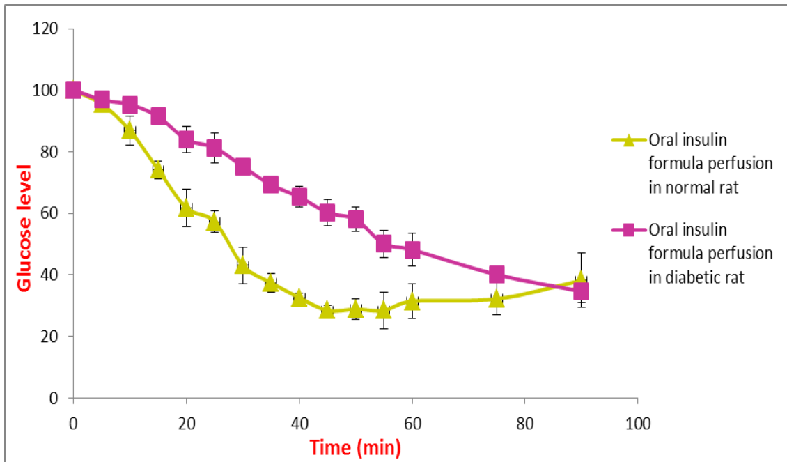
(Figure 3.17): Comparison percentage of blood glucose levels between normal and diabetic rats after in situ oral insulin formula perfusion. (Data is as mean \pm SEM).
