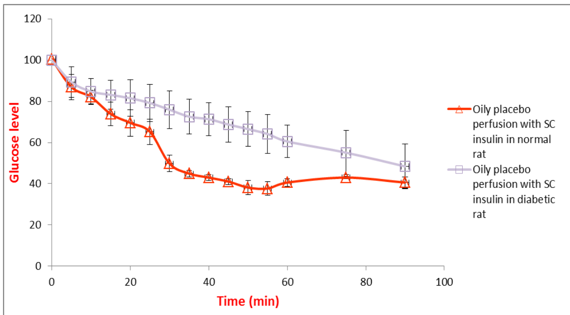
(Figure 3.18): Comparison percentage of blood glucose levels between normal and diabetic rats after in situ oily placebo perfusion with SC insulin injection (1IU/ml). (Date is as mean \pm SEM).
